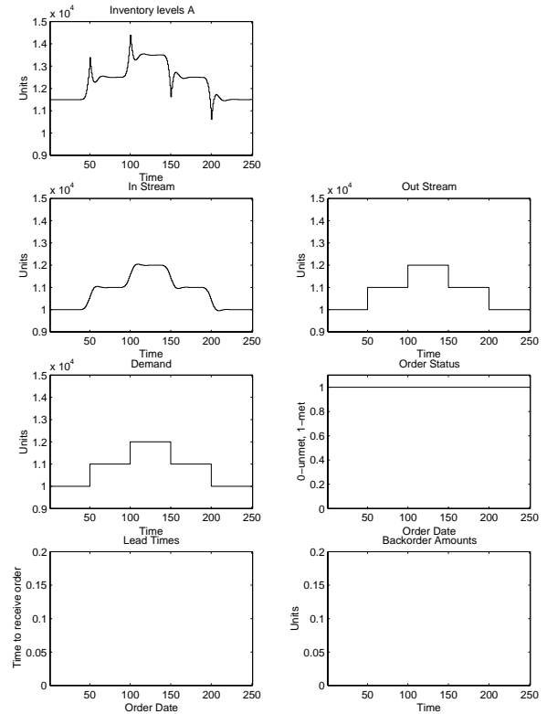
Figure 5: Retailer Responses and Metrics, Two-Node Example, With Move Suppression
