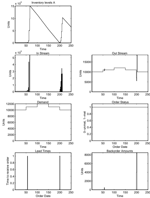
Figure 4: Retailer Responses and Metrics, Two-Node Example, No Move Suppression
