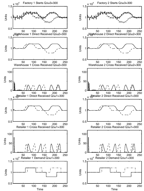
Figure 10: Material flows Product A (dashed) and Product B (solid); Demand: Product A (dotted) and Product B (dash-dot) and corresponding customer receipts Product A (dashed) and Product B (solid).
