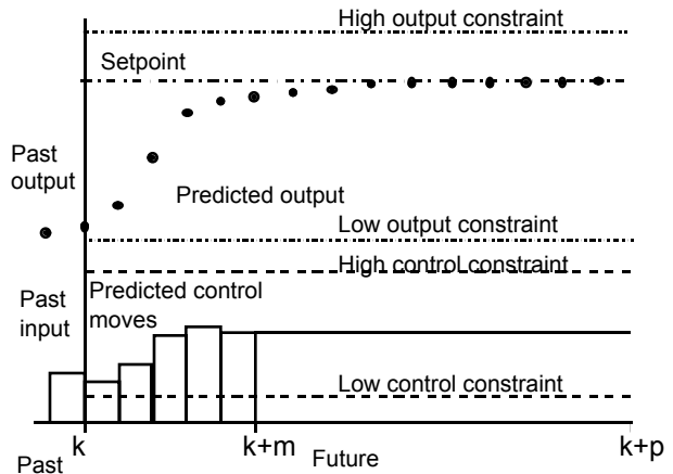
Figure 1: MPC receding horizon philosophy.
