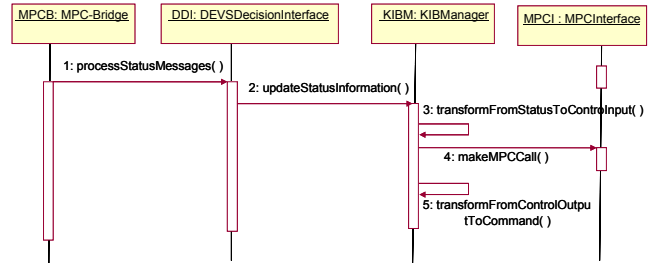
Figure 10: Data and Control Mapping Snippet
