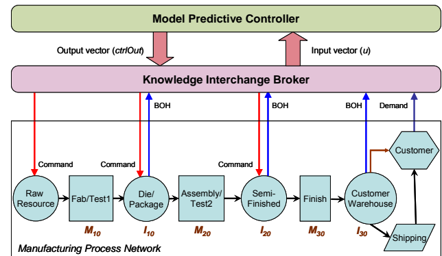
Figure 5: Composition of Manufacturing Process Network and MPC via KIB
