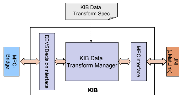
Figure 7: Software Components in KIB
