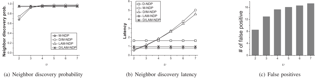
Fig. 8. The impact of \nu on the neighbor discovery probability, latency and false positives of M-NDP.
