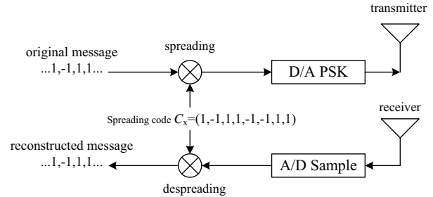
Fig. 1. A simplified system diagram of DSSS.
