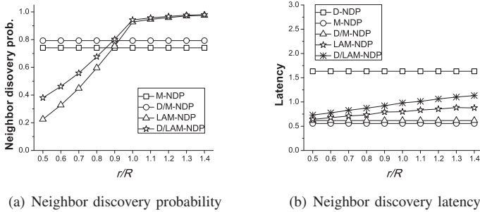
Fig. 9. The impact of propagation range on the neighbor discovery probability and latency of LAM-NDP.
