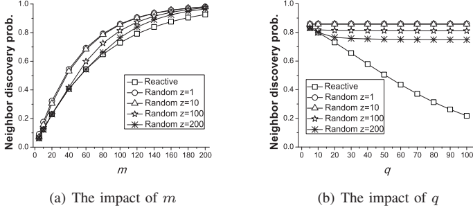
Fig. 6. D-NDP under reactive and random jamming attacks.
