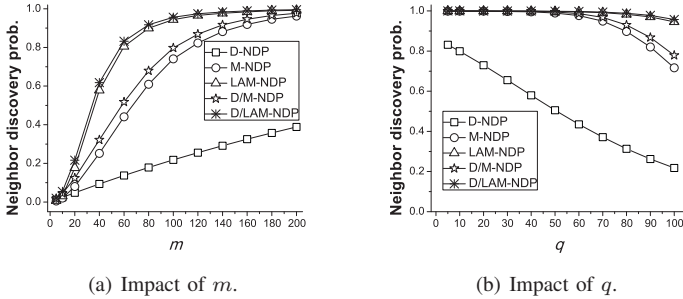
Fig. 7. Comparison of the neighbor discovery probabilities of different protocols.
