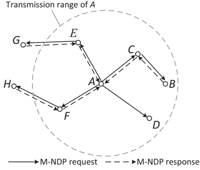
Fig. 2. Illustration of M-NDP.
