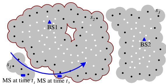
Fig. 1. An exemplary WSNs. There are three sensor clusters: Clust(s_1) , Clust(s_2) , and Clust(s_3) , two static BSs: BS1 and BS2 and one mobile BS: MS. Shaded area, solid dots and open dots represent the coverage of sensors, boundary nodes and interior nodes, respectively. The boundary of Cover(s_2) is depicted by red curves.
