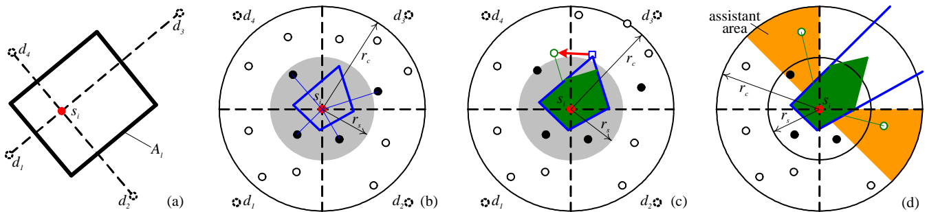
Fig. 2. Illustration of the LVP-based boundary node detection algorithm.
