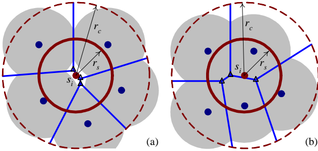
Fig. 13. Voronoi-diagram based coverage hole prediction.
