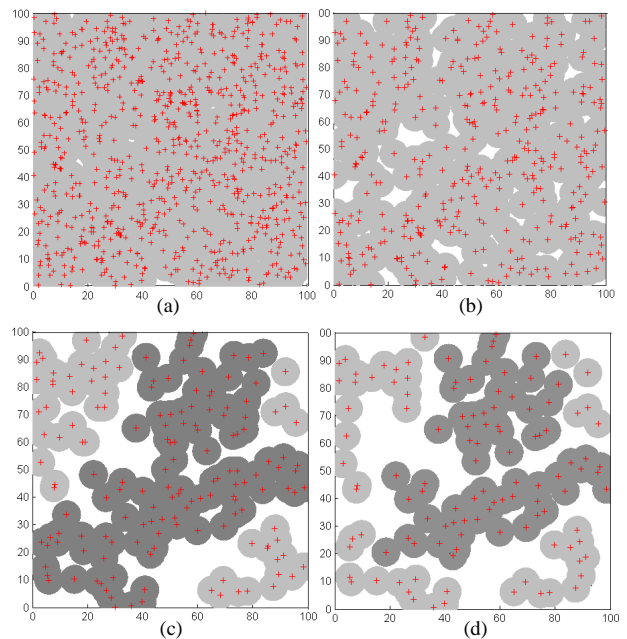
Fig. 14. Some network topologies used in our performance evaluation. (a) k = 40 . (b) k = 15 . (c) k = 5 . (d) k = 4 . In all situations, the position of the BS is (50, 50). Shaded area represents coverage of sensors. Notice that in (c) and (d) only darkly shaded area represents connected coverage needed to be measured.
