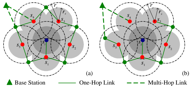
Fig. 4. Non-locality of the boundary node detection when r_c < 2r_s .
