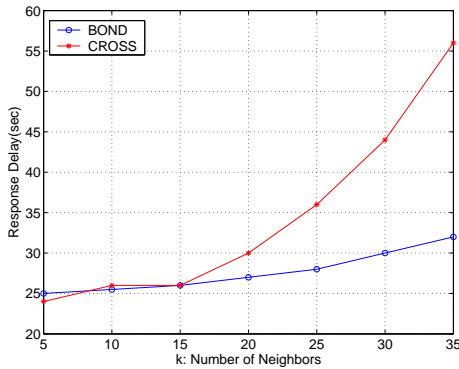
Fig. 9. Simulation results with T_{EUP} = 10s , Pr[FA] \leq 0.01 .
