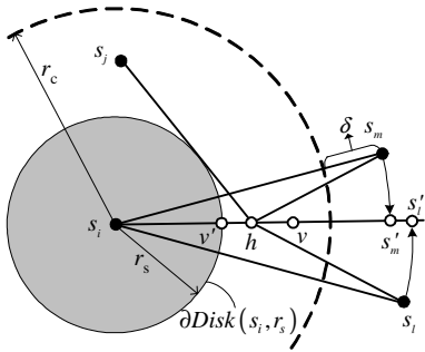
Fig. 3. Illustration of the proof of Theorem 1.
