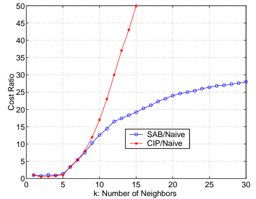
Fig. 12. Energy cost ratio of SAB and CIP to naive scheme.
