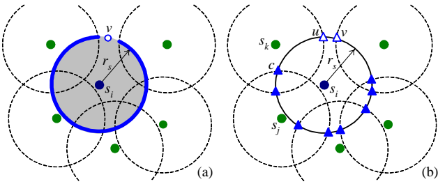
Fig. 7. Perimeter-based boundary node detection approaches. (a) Perimeter-coverage checking approach proposed in [16]. The solid curve represents the portion of perimeter of sensing disk covered by neighbor nodes. (b) Crossing-coverage checking approach proposed in [13], [42]. Solid and open triangles represent covered and uncovered crossings, respectively.
