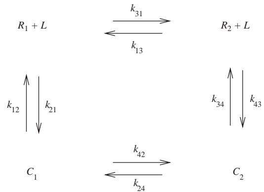
Fig. 1. A two-state receptor–ligand network.
