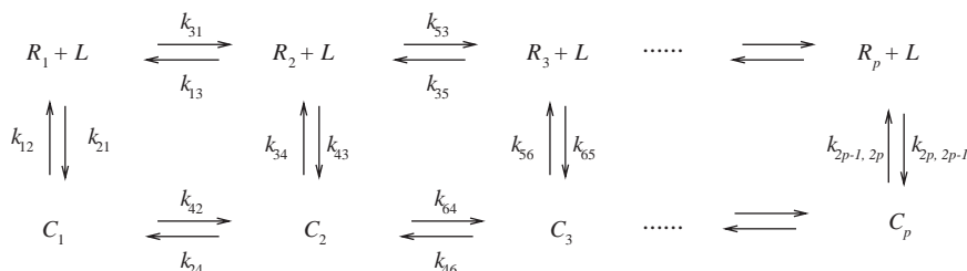
Fig. 5. A “ladder” receptor–ligand network, incorporating p receptor conformations.
