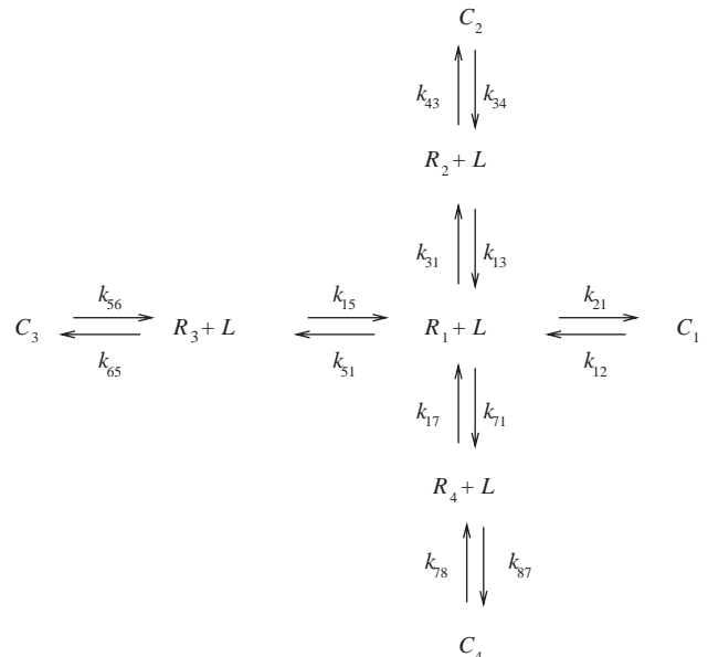
Fig. 6. A ‘‘star’’ receptor–ligand network.
