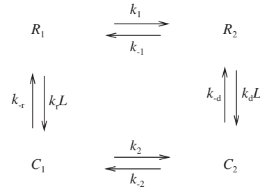
Fig. 4. The model studied in Segel et al. (1986).
